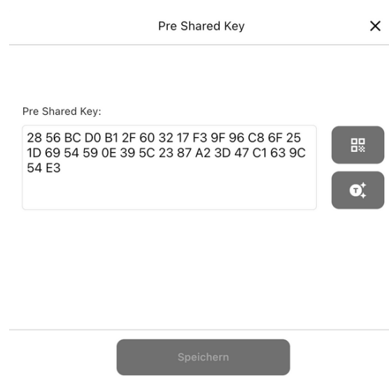
Figure 3: Add the PSK to the App
