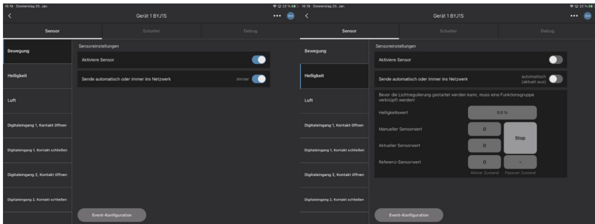
Figure 14: Step 3 (left) – activating “send always to mesh” of the motion sensor and step 4 (right) – brightness menu.
