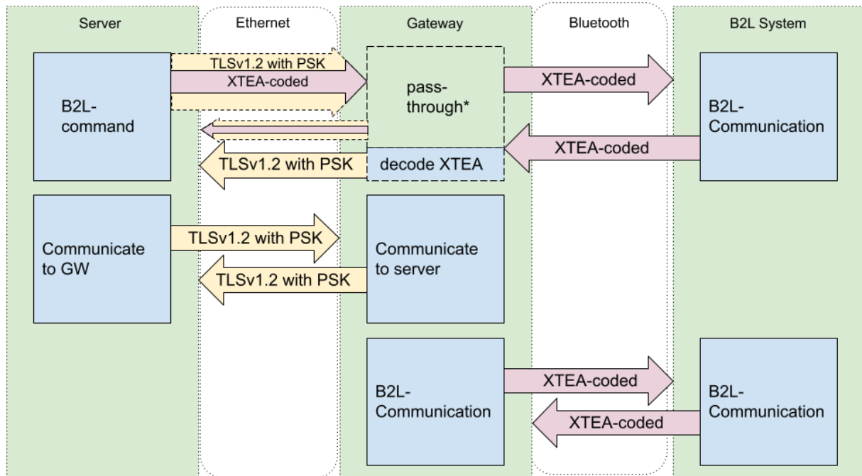
Figure 28: Visualization of the XTEA-algorithm in B2L
